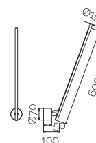
9081 WALL 600
