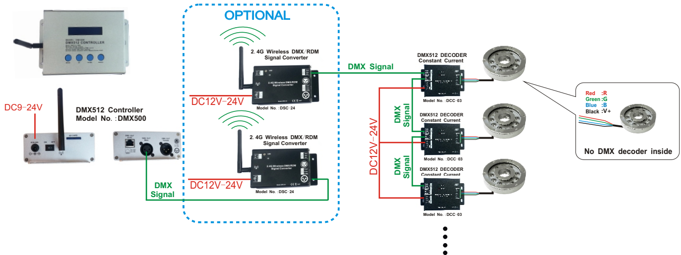
Wiring Diagram (1)
