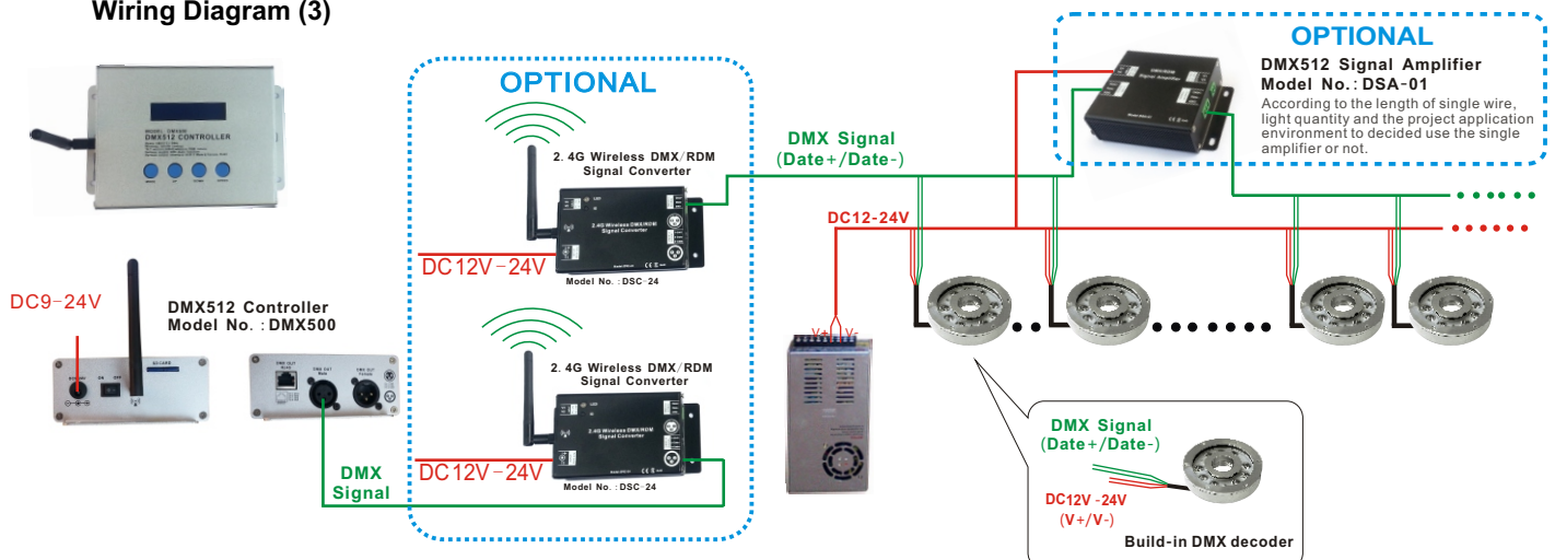
Wiring Diagram (3)
