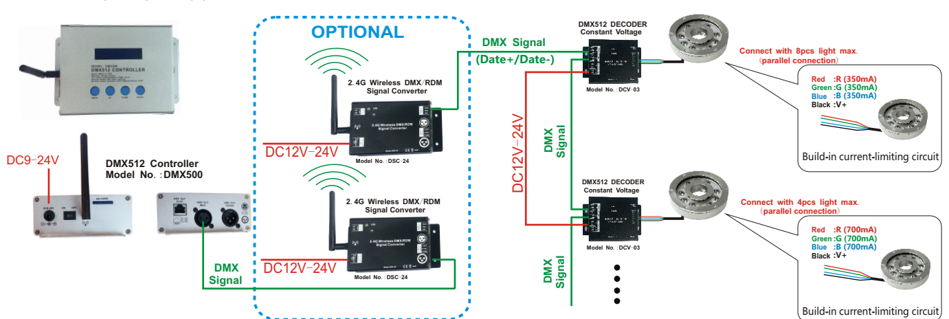
Wiring Diagram (2)
