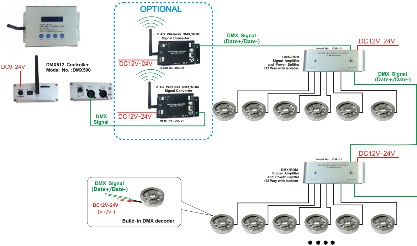
Wiring Diagram (4)
