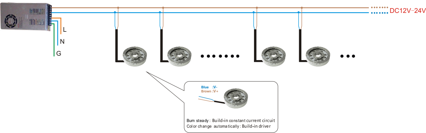
Wiring Diagram (5)
