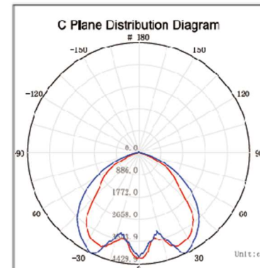
Light Distribution Curve
