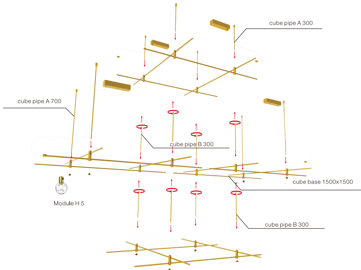
Ⓐ Module H 5 quick installation
