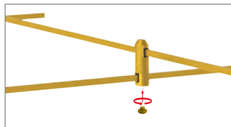
Ⓓ Bottom cover rubber plug installation
